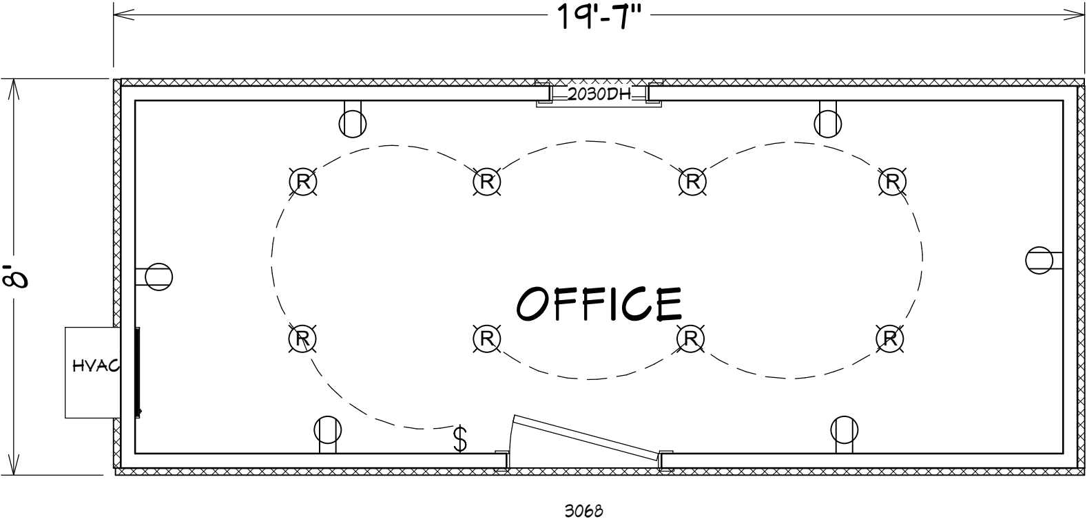
20' Office Layout
